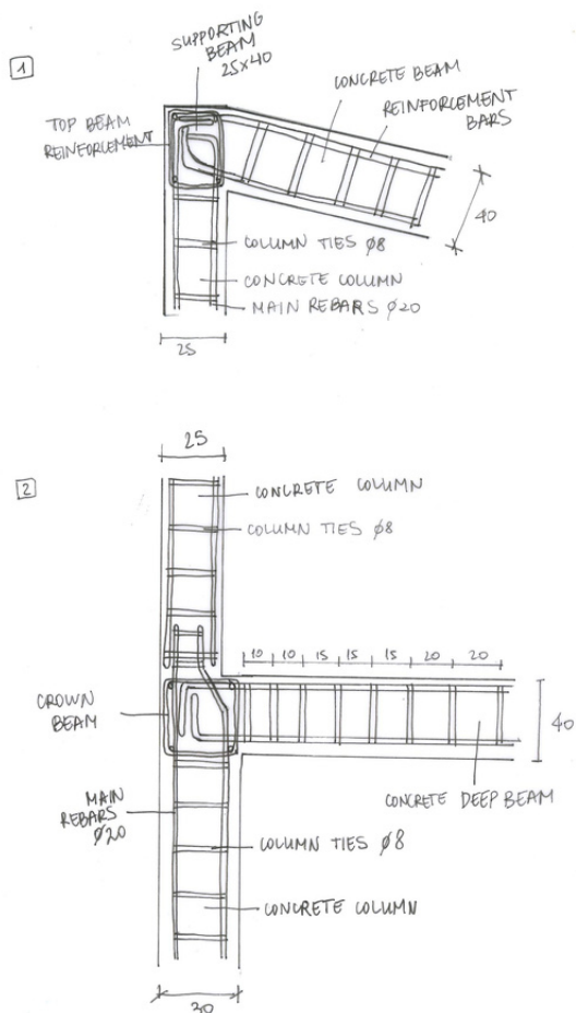
CONSTRUCTION DETAILS 1/20
