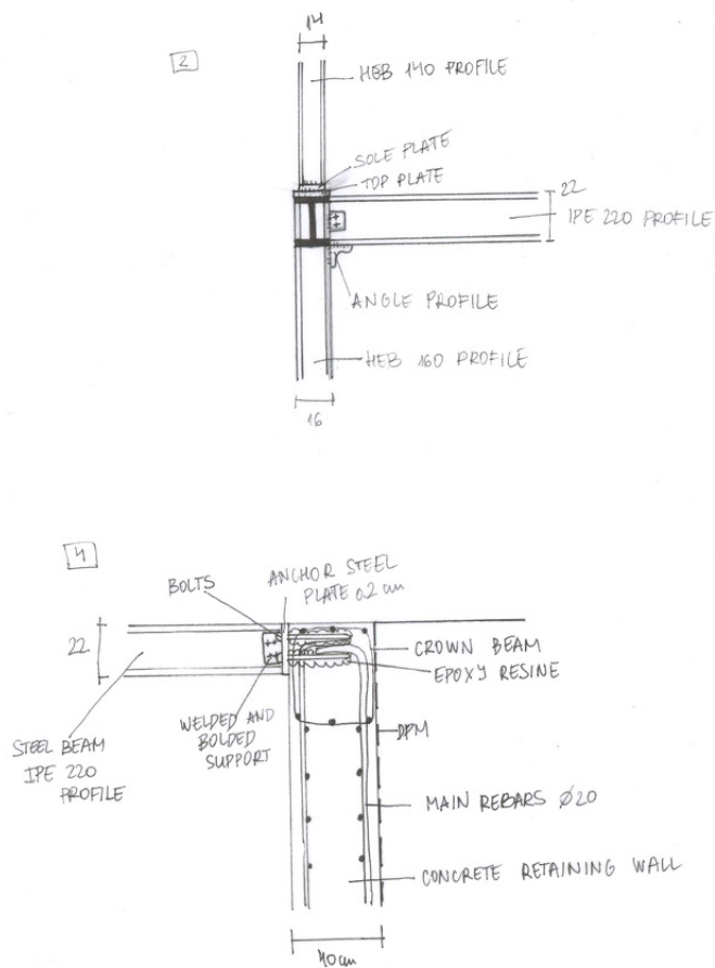
CONSTRUCTION DETAILS 1/20
