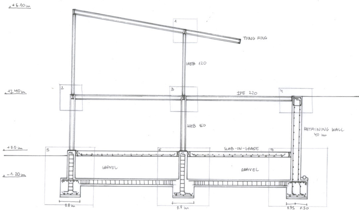
SECTION 1/50
