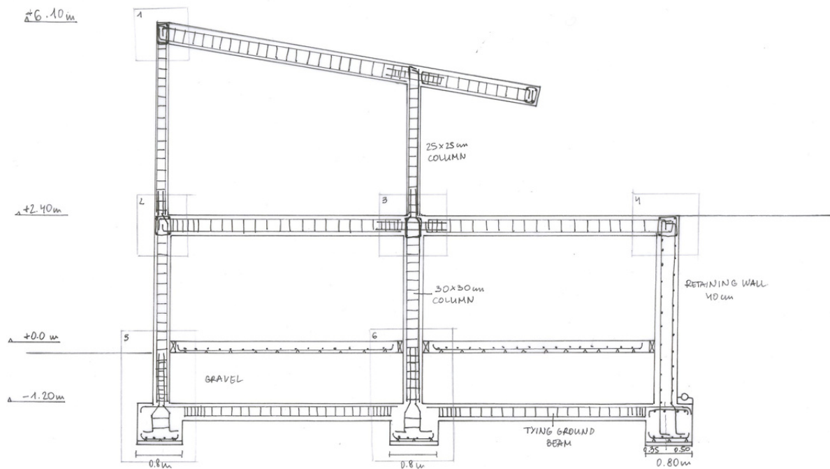
SECTION 1/50
