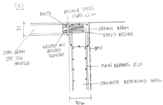
CONSTRUCTION DETAILS 1/20
