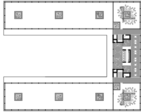
Roof floor plan
