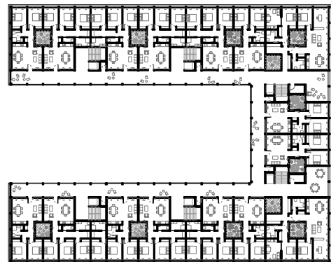
Common floor plan
