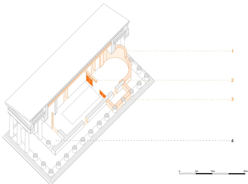
Fig. 3 - Exploded Axonometry of the Theseion temple, at Christian stage.
