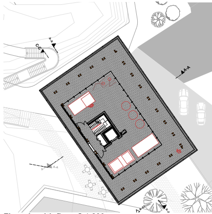
Floorplan 4th floor S 1:200
