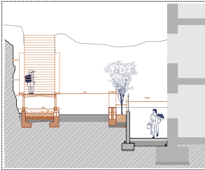
Section Extract _ 1:50
