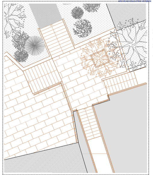
Plan Extract _ 1:50
