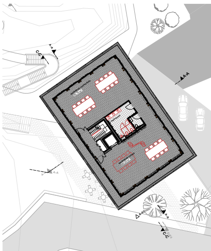
Floorplan 7th floor M 1:200
