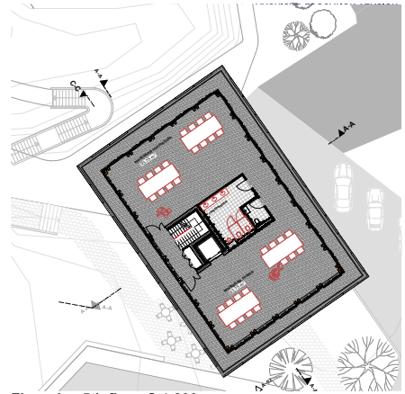
Floorplan 5th floor S 1:200
