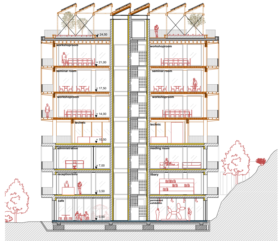
Zoom-In Section C S 1:100
