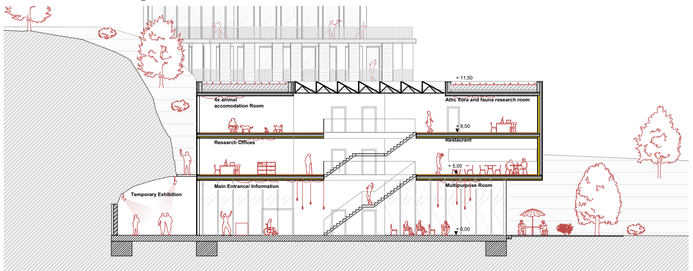
Section B S 1:100
