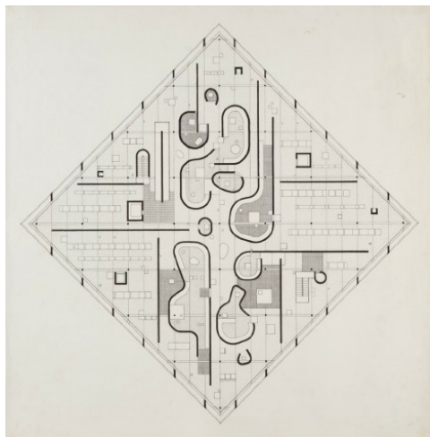
Fig. 6 John Hejduk, Diamond Houses , House B - 1967
