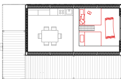
Plan mezzanine
